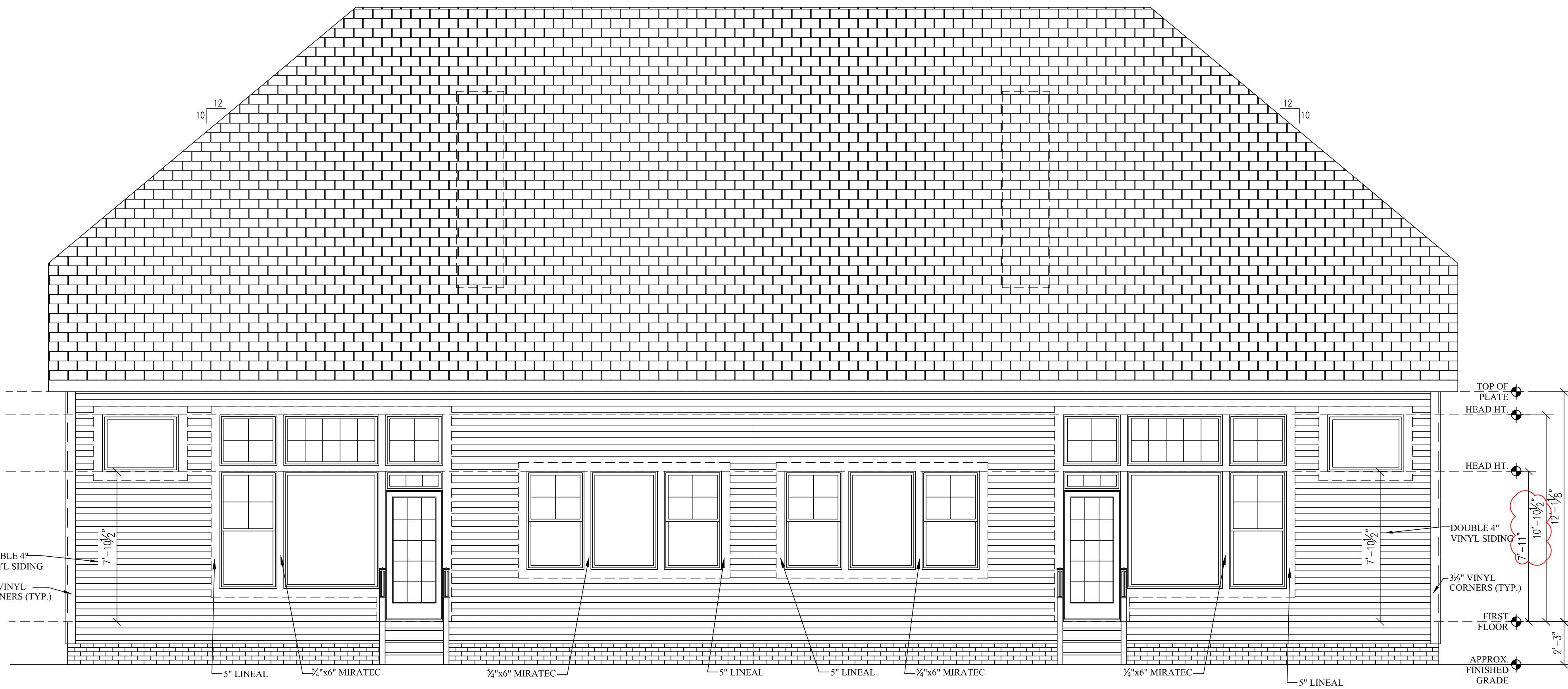
REAR ELEVATION ELEVATION B Scale: 1/4" = 1'-0"
